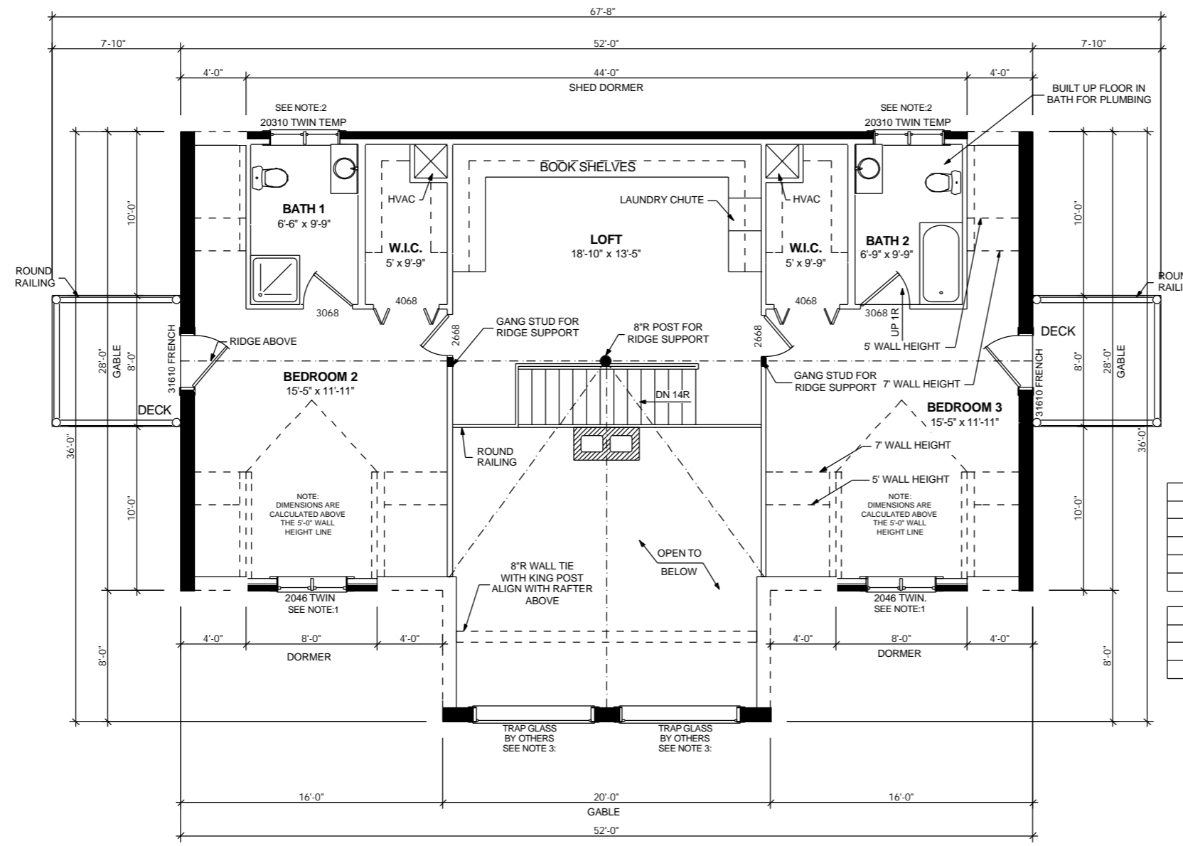
2nd FLOOR PLAN Scale : 1/4" = 1'-0"
