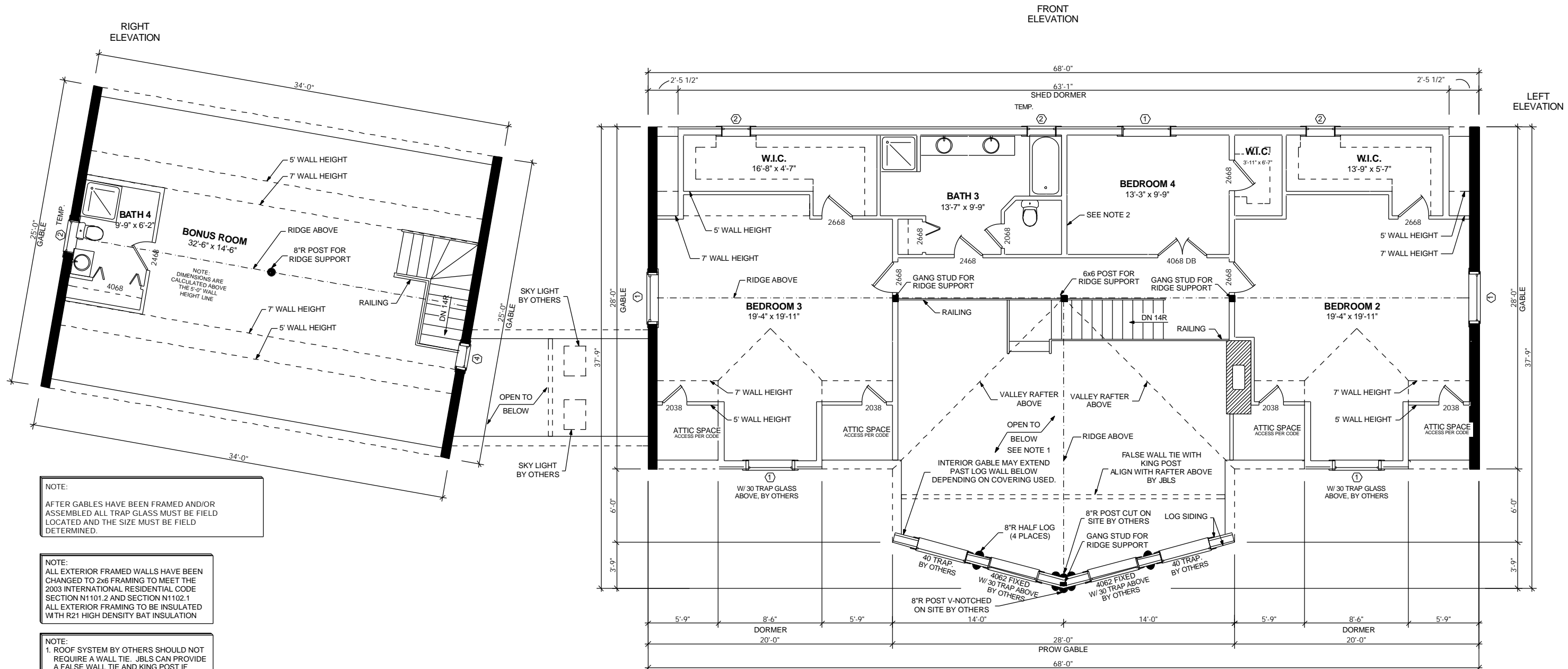
2nd FLOOR PLAN Scale: 1/4" = 1'-0"
