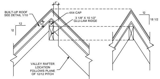
A 9 ROOF DETAIL Scale : 3/4" = 1'-0"
