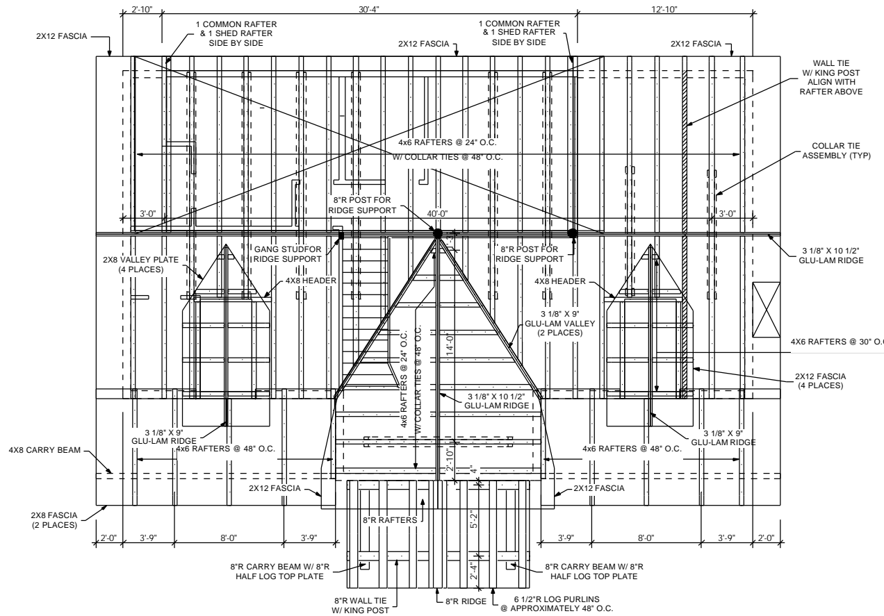
ROOF FRAMING Scale : 1/4" = 1'-0"
