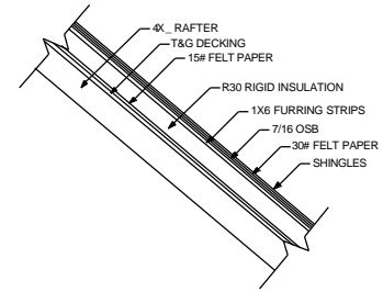
1 BUILT-UP ROOF DETAIL Scale: 3/4" = 1'-0"
