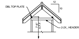
2 GABLE DORMER HEIGHT Scale: 1/4" = 1'-0"
