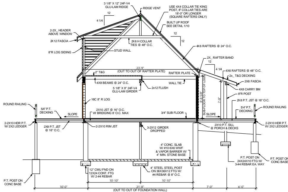
A BUILDING SECTION "A" Scale: 1/4" = 1'-0"
